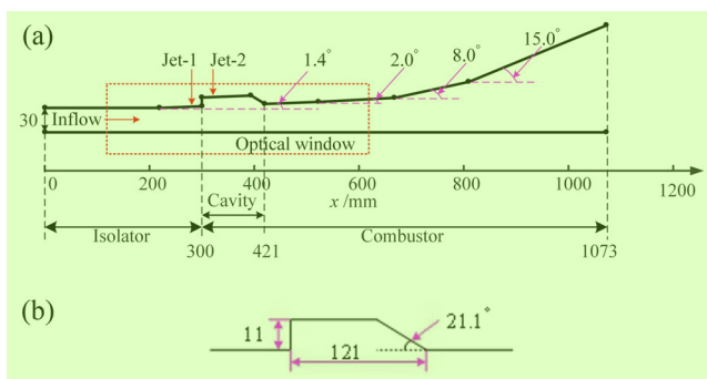
FIG. 2. Geometric configurations of (a) the tested combustor and (b) cavity.
