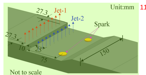
FIG. 3. Schematic of fuel injection and spark.
