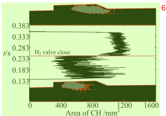
FIG. 16. Area of the CH region in case 6. 7
