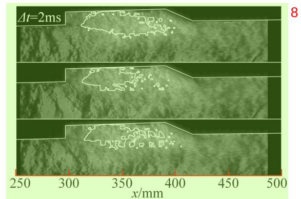
FIG. 17. Schlieren images and the CH region in the presence of the H_2 pilot flame. 9
