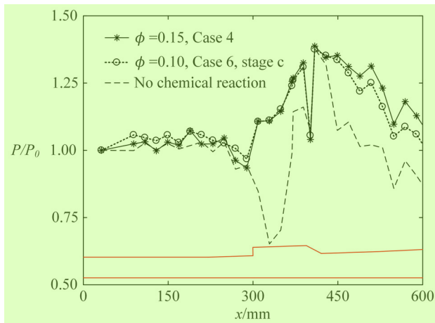
FIG. 19. Normalized pressure distributions with pure C_2H_4 .
