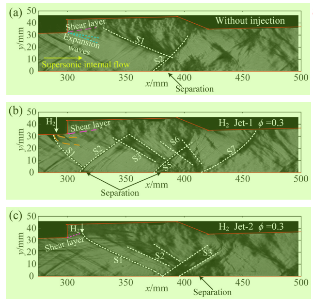
FIG. 7. Internal structures of supersonic flow under various injection strategies: (a) non-reacting flow; (b) hydrogen injected at Jet-1 location; and (c) hydrogen injected at Jet-2 location. 11
