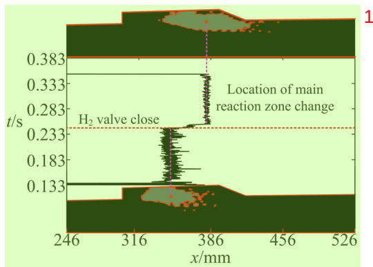
FIG. 15. X coordinate of the center of CH region in case 6. 2
