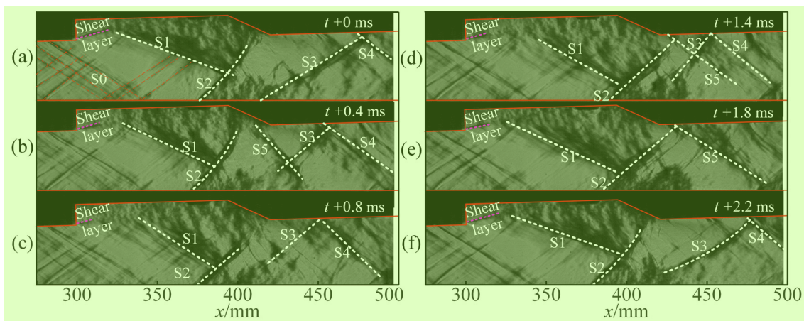
FIG. 6. Internal supersonic flow structures without fuel injection. 13
