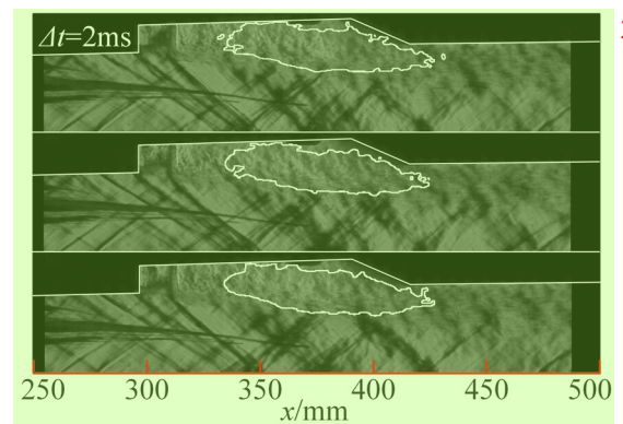
FIG. 18. Schlieren images and the CH region without H_2 pilot flame. 14
