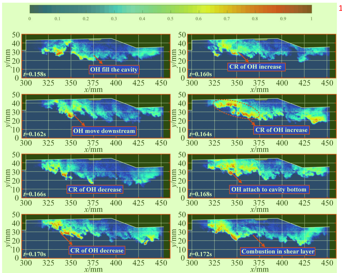
FIG. 9. OH-PLIF images of cavities with pure H_2 at \phi = 0.3 injected at Jet-1.
