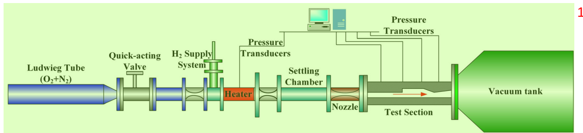
FIG. 1. Schematic of a direct-connected pulse combustion wind tunnel.
